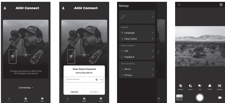
FIGURE 2-7. CLIENT SOFTWARE
